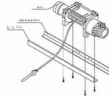
The mounting drawing of YD type
